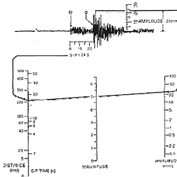
Figure 5-11: Richter Scale
