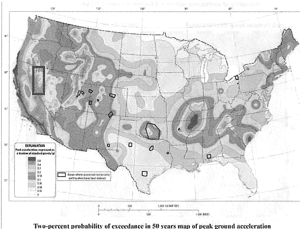
Figure 5-14: Peak Ground Acceleration (%g) with Two Percent (2%) Probability of Exceedance in 50 Years
