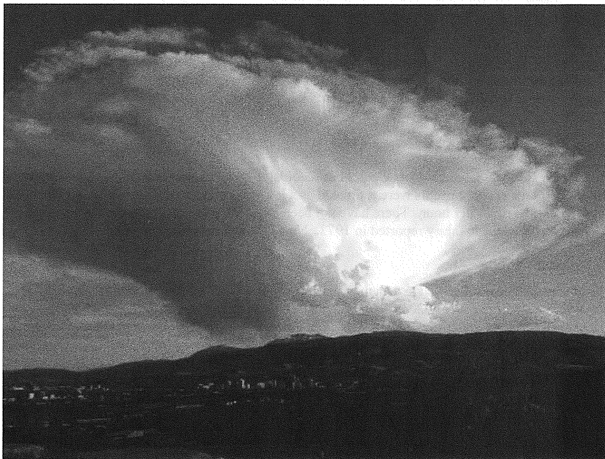
Figure 5-23: Thunderstorm over Incline (June 4, 2013)
