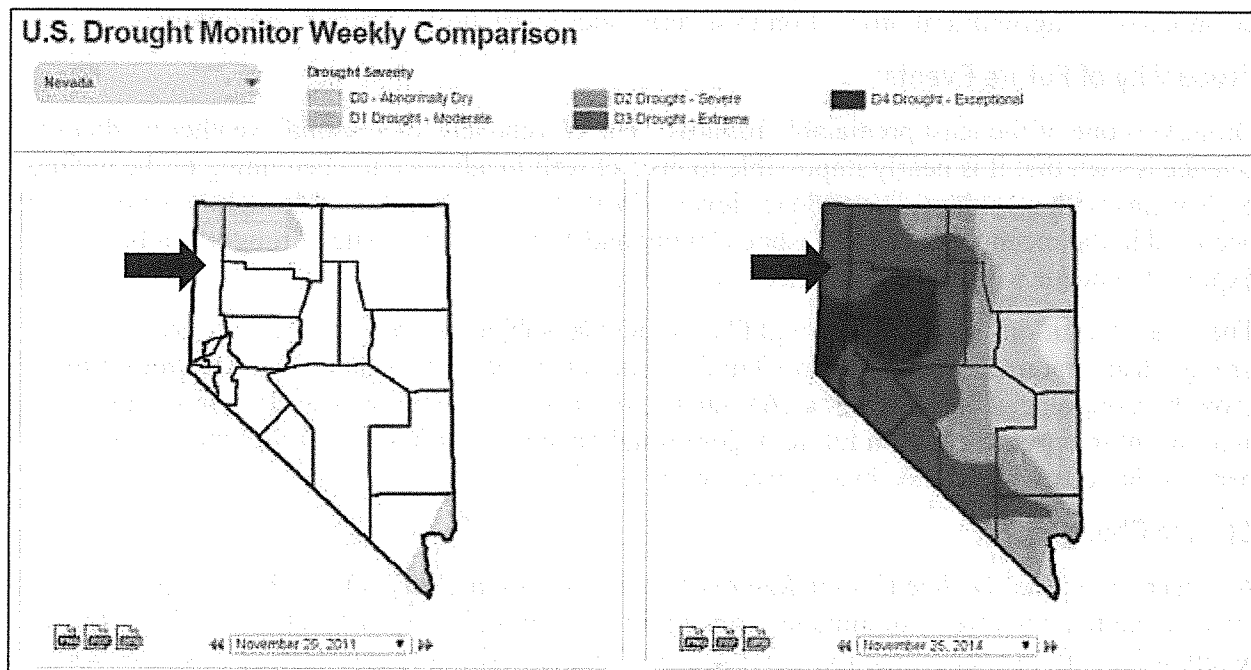
Figure 5-10: US Drought Monitor for Nevada November 2011 vs. November 2014
